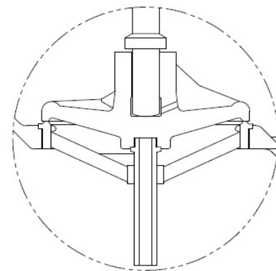
Screw-down check valve
